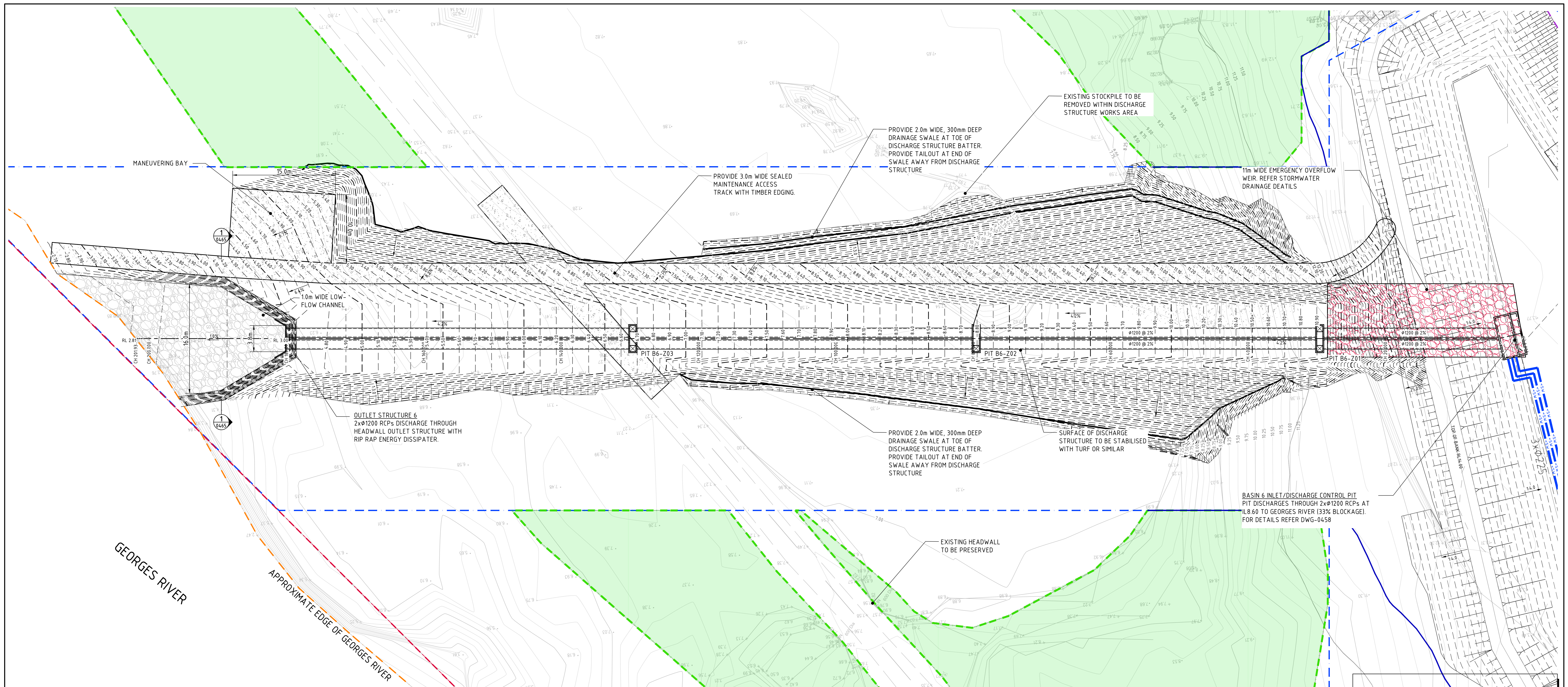
BASIN 6 OUTLET STRUCTURE PLAN 1:200 SCALE
