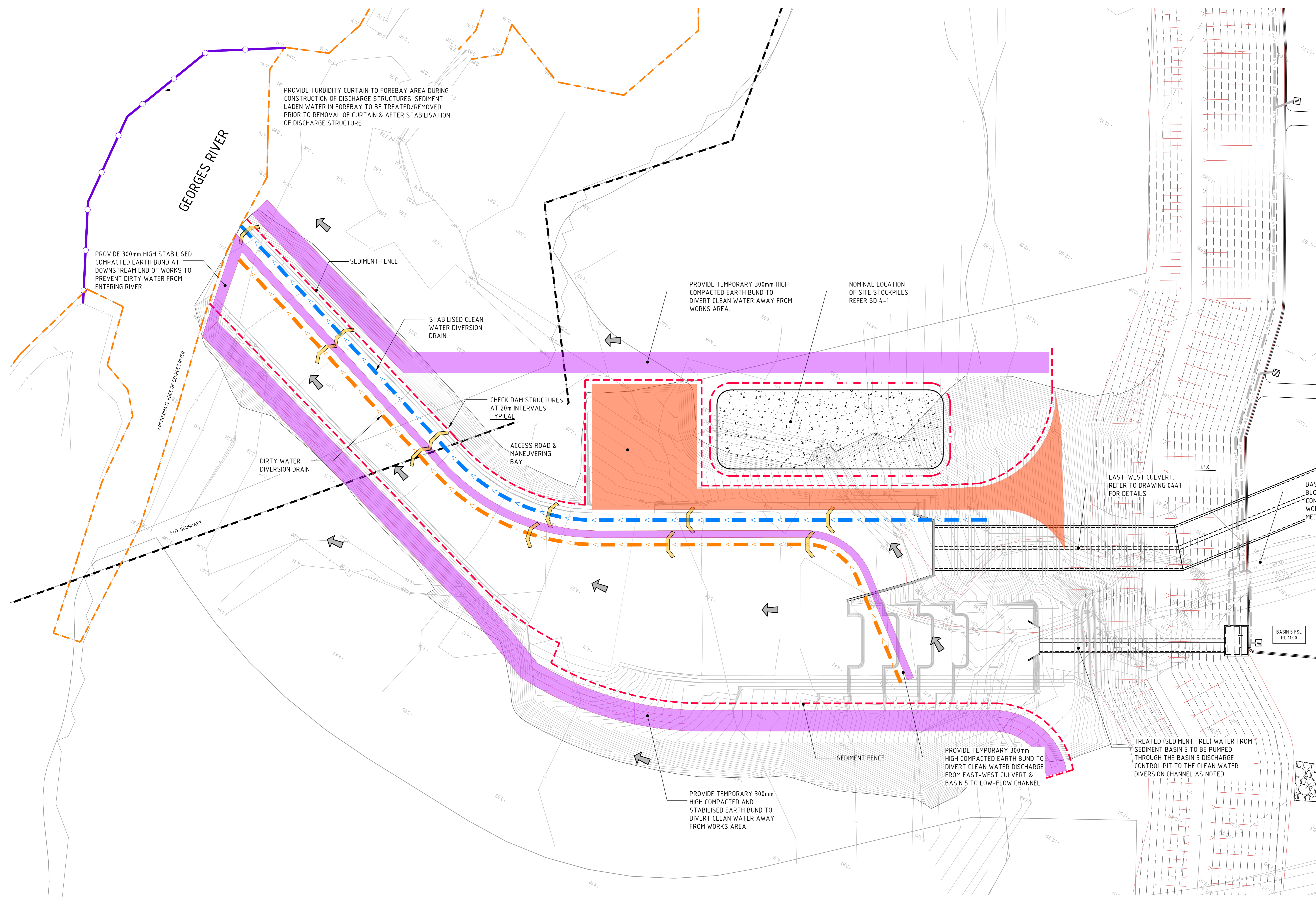
BASIN 5 OUTLET EROSION & SEDIMENT CONTROL PLAN 1:200 SCALE
