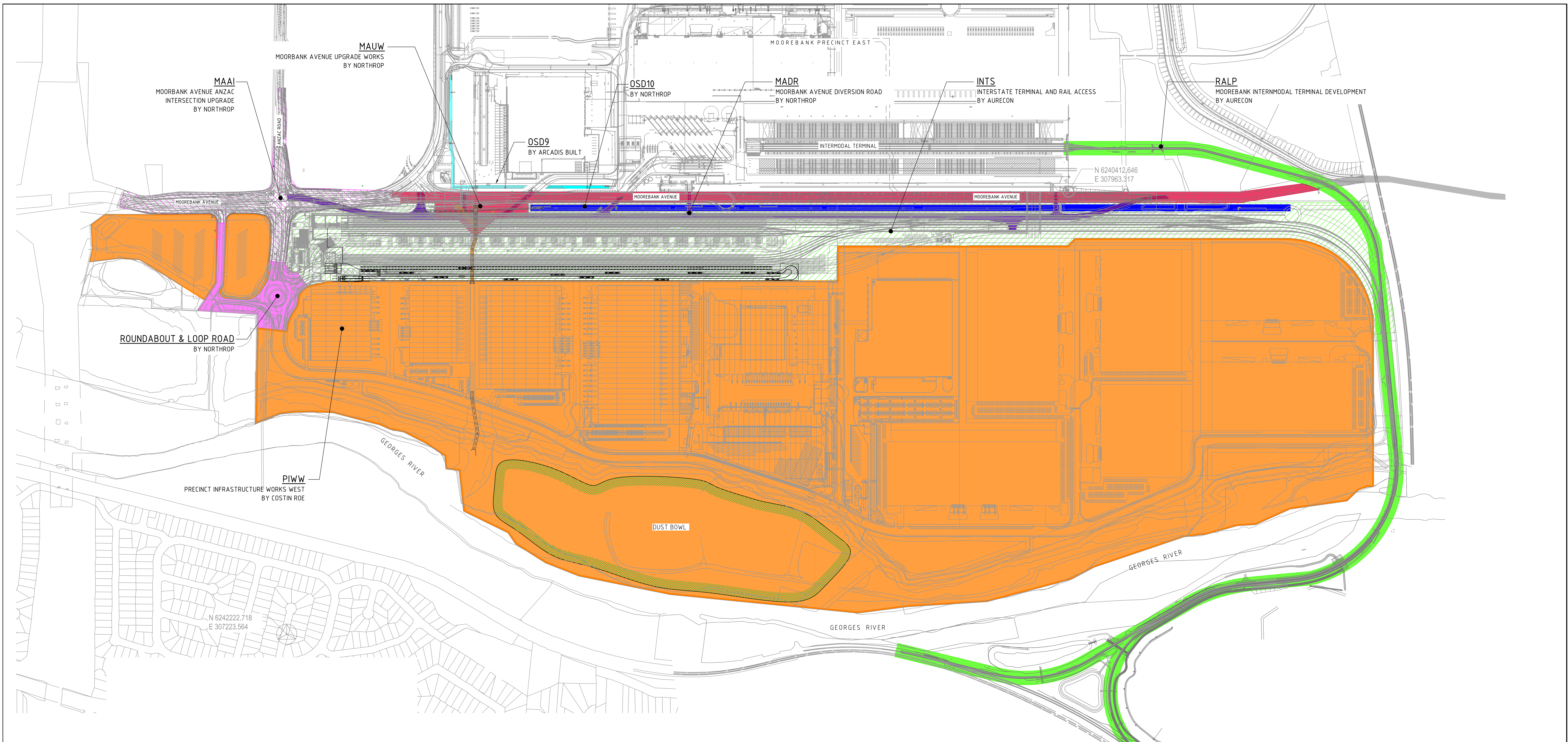
MPW GENERAL WORKS SITE ARRANGEMENT PLAN 1:3000 SCALE
