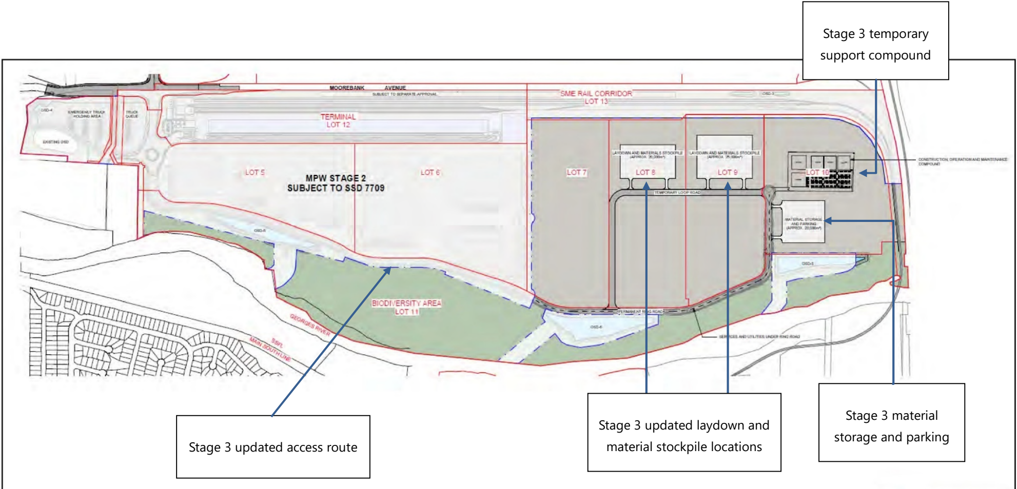
Figure 1 – Proposed MPW Stage 3 development works area and layout
