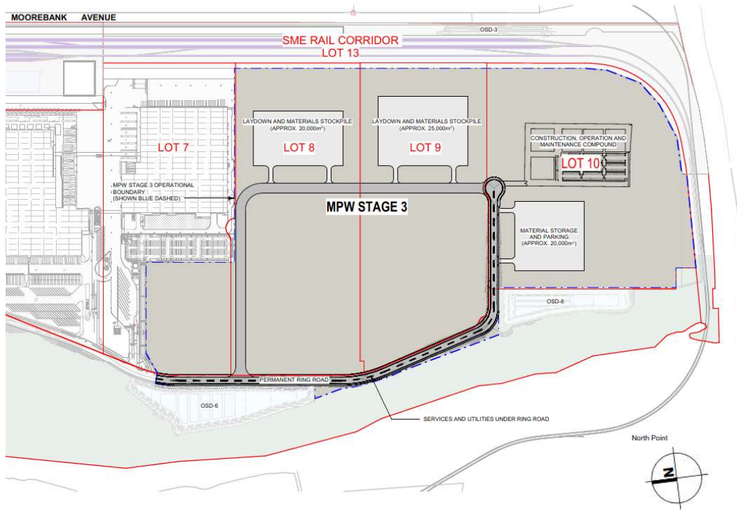
Figure 4 – Development Construction Compounds, Stockpiles and Construction Area (MPWS3) (refer to Figure 1 for context map)
