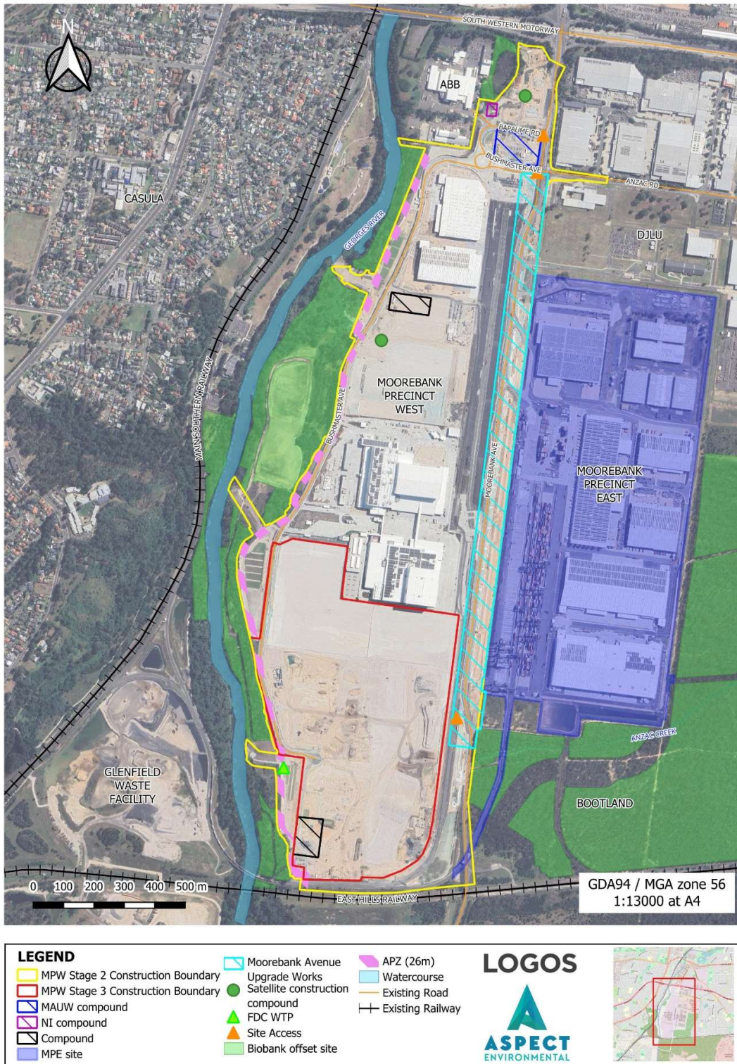
Figure 3 – Development Construction Compounds, Stockpiles and Construction Area (MPWS2)
