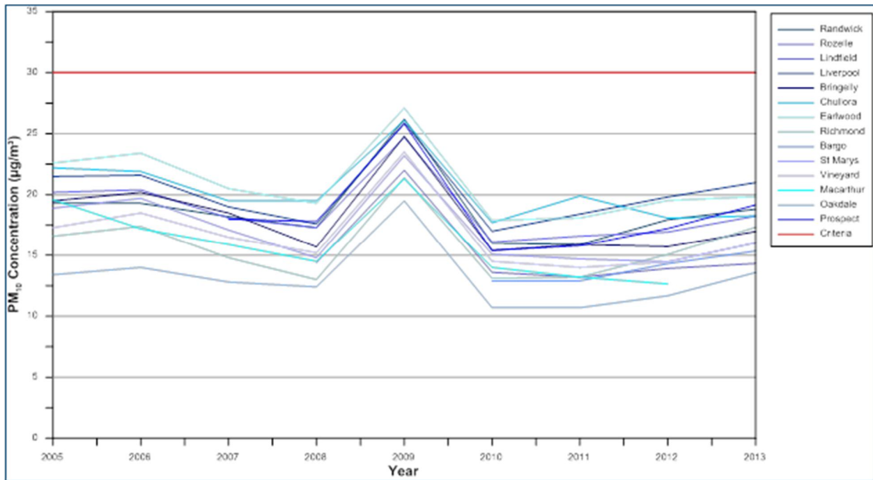
Figure 18.3 Annual average \text{PM}_{10} concentrations at NSW EPA monitoring sites
