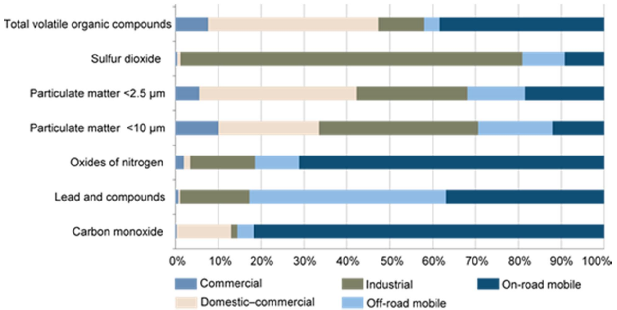
Figure 18.1 Sydney's total estimated annual emissions by source type
